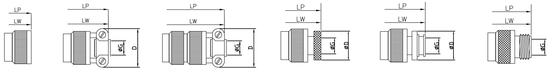
GROMMET SEAL WITH BACK NUT [E] GROMMET SEAL WITH STRAIN RELIEF [F] WATER TIGHT GLAND SEAL WITH STRAIN RELIEF FOR JACKETED WIRE [J] GROMMET SEAL WITH BACK SHELL FOR HEAT SHRINK [H] GROMMET SEAL WITH BACK SHELL FOR SCREEN TERMINATION [S] THREADED ADAPTOR SHELL FOR CABLE ACCESSORIES, EXPOSED SOLDER BUCKETS [T]
