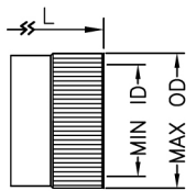
GROMMET SEAL WITH BACK NUT [E]
